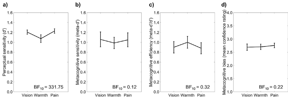
Fig. 2. Mean values of (a) perceptual sensitivity, i.e. d' , (b) metacognitive sensitivity, i.e. \text{meta-}d' , (c) metacognitive efficiency, i.e. \text{meta-}d'/d' , and (d) metacognitive bias, i.e. mean confidence, in the visual contrast, innocuous warmth, and nociceptive pain discrimination tasks. A Bayes factor ( \text{BF}_{10} ) > 3.00 indicates differences between conditions. A \text{BF}_{10} < 0.33 indicates no differences between conditions. Error bars show 95% credible intervals (CI).
